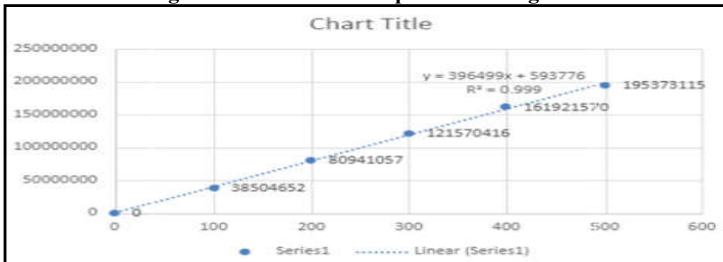
Figure No.5: Calibration plot of Lamivudine
