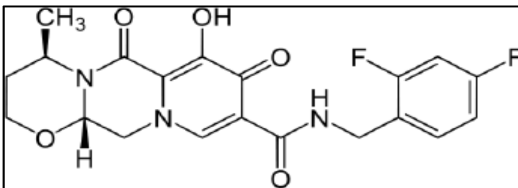
Figure No.2: Chemical structure of Dolutegravir
